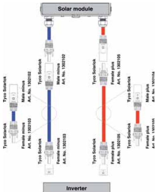
Tyco Solarlok connectors 4 mm²
