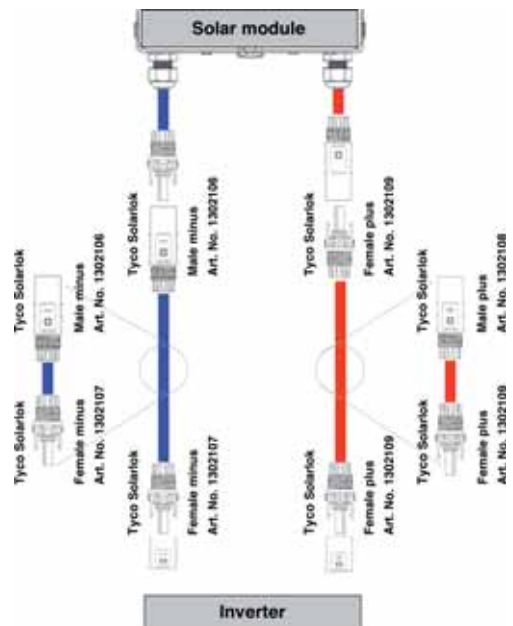
Tyco Solarlok connectors 6 mm²
