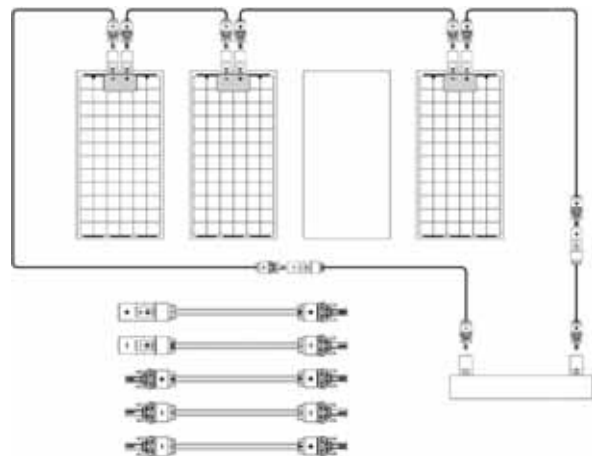
With the Tyco Solarlok system the female and the male are both available with Plus and Minus configuration.
